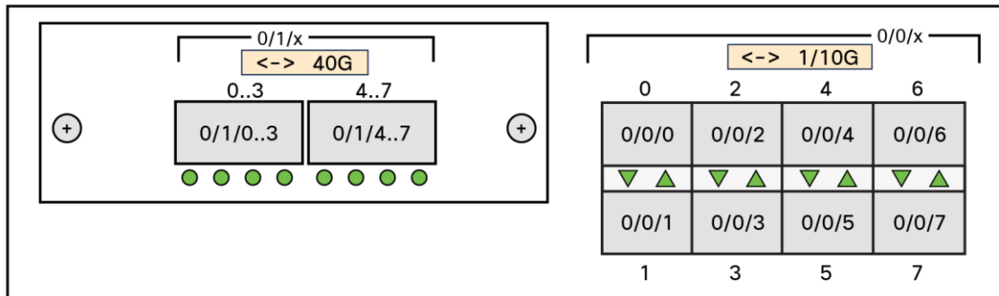
Figure 8. CW9800H2 port identification
